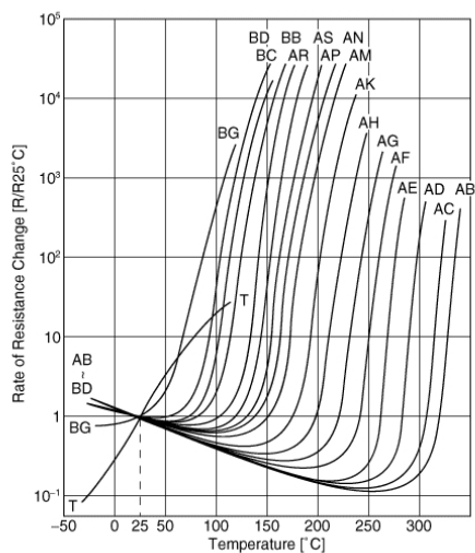
Resistance-Temperature Charac.
