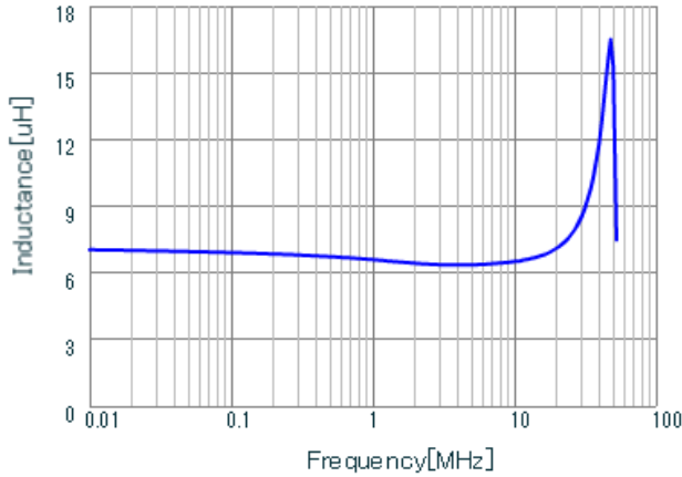
LQH44PN6R8MP0 L
