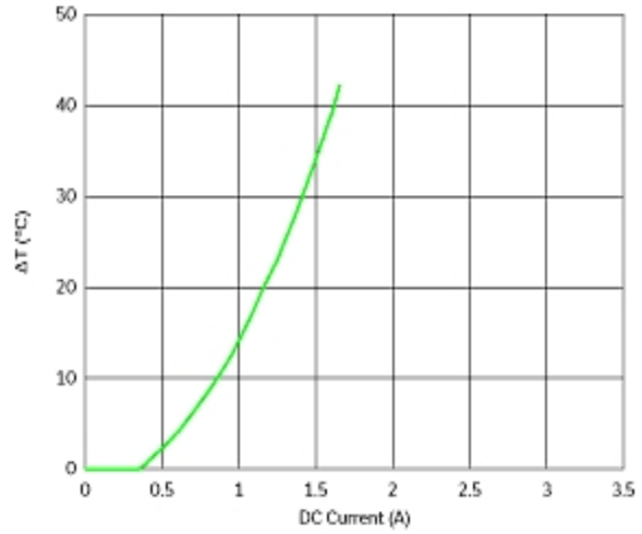
Temperature Increase Characteristic
