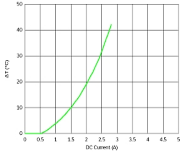
Temperature Increase Characteristic
