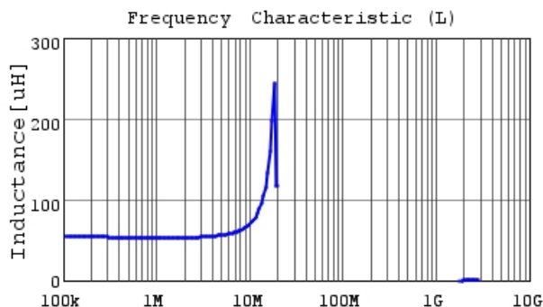
LQH32NH560J23 L
