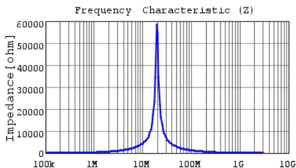
LQH32NH560J23 |Z|
