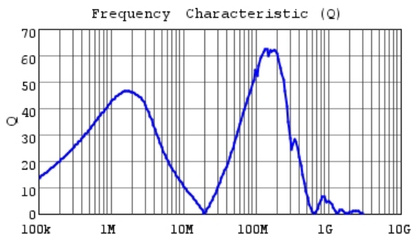
LQH32NH560J23 Q
