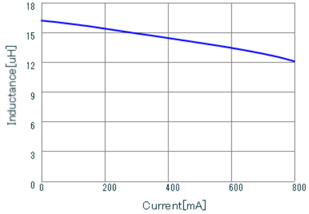
LQH32PN150MNC DC-Bias, 20
