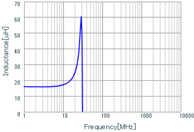
LQH32PN150MNC L
