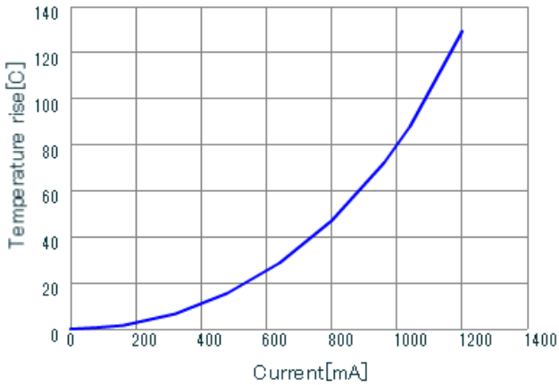
LQH32PN150MNC DT_Current
