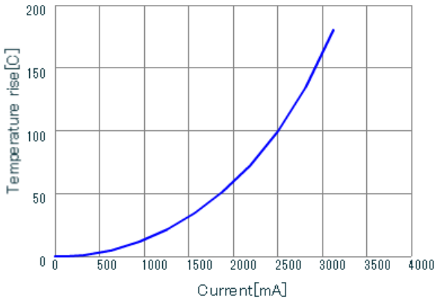
LQH3NPN4R7MGR DT_Current
