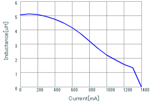
LQH3NPN4R7MGR DC-Bias, 20
