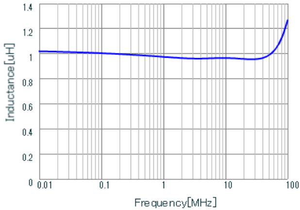
LQH44PN1R0NP0 L
