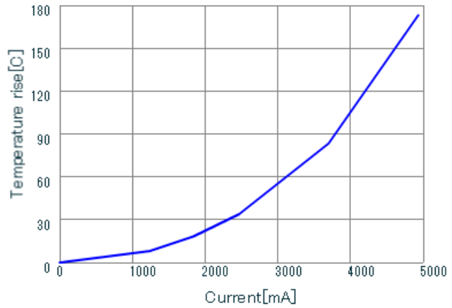
LQH44PN1R0NP0 DT_Current
