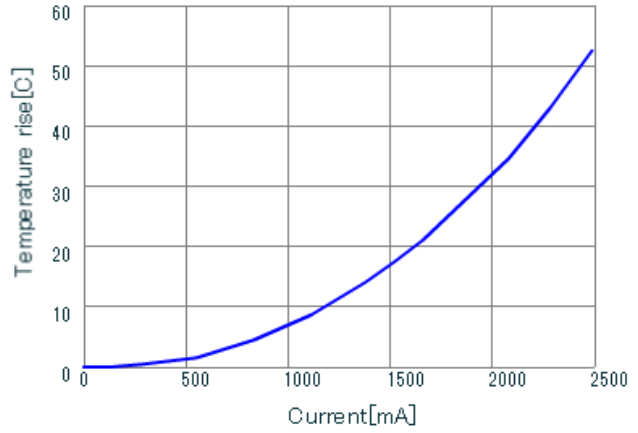
LQH44PN1R5MJ0 DT_Current
