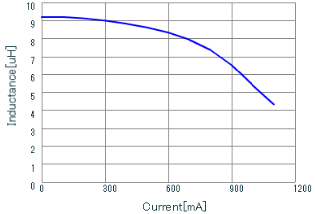
LQH44PZ100MGR DC-Bias, 20
