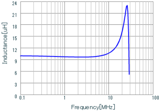
LQH44PZ100MGR L
