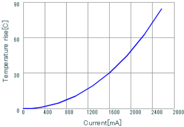
LQH44PZ4R7MGR DT_Current
