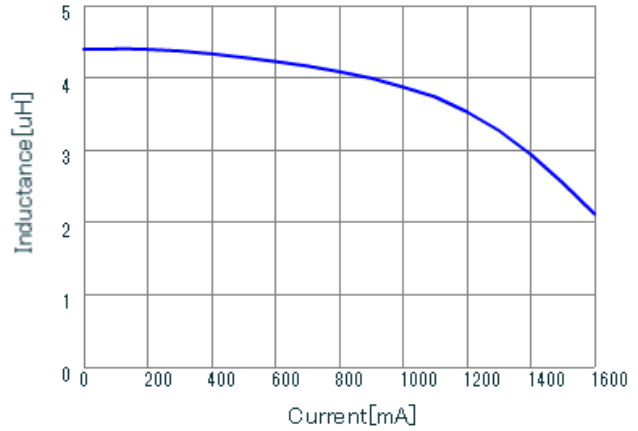
LQH44PZ4R7MGR DC-Bias, 20
