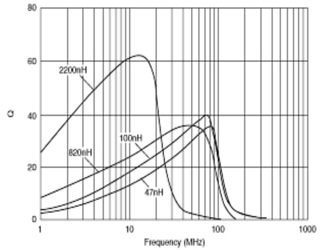
Q-Frequency Characteristics
