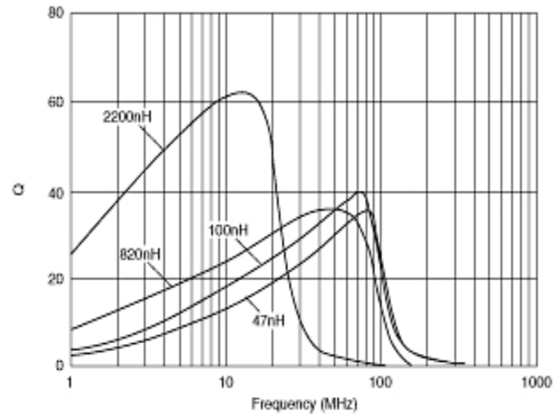
Q-Frequency Characteristics
