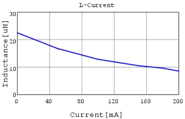
LQM21DN220M70 L-Current 20degC
