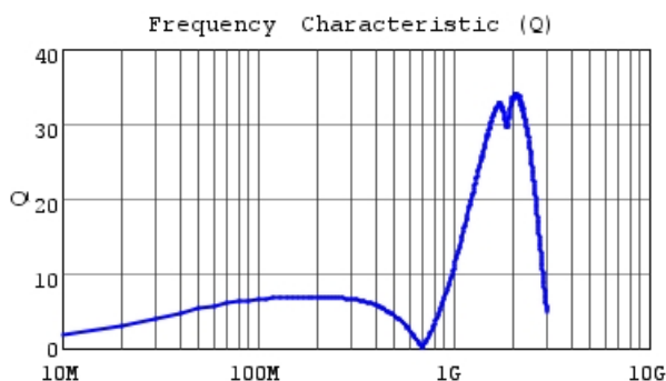
LQP03TNR22J02 Q
