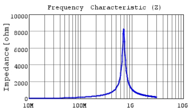
LQP03TNR22J02 |Z|
