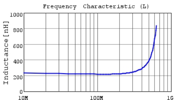
LQP03TNR22J02 L
