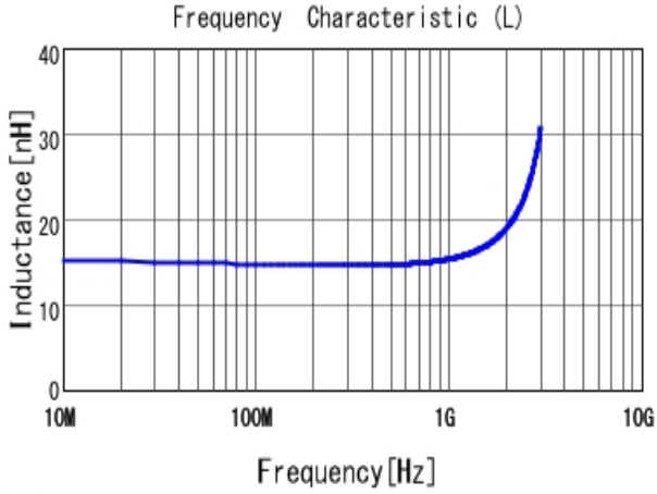
■ LQW2BAS15NJ00 L
