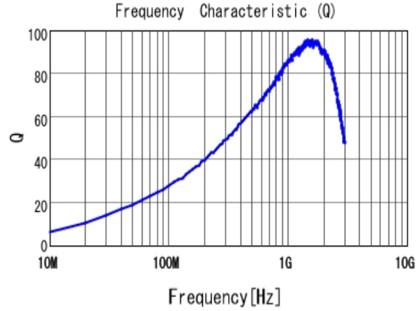
■ LQW2BAS15NJ00 Q
