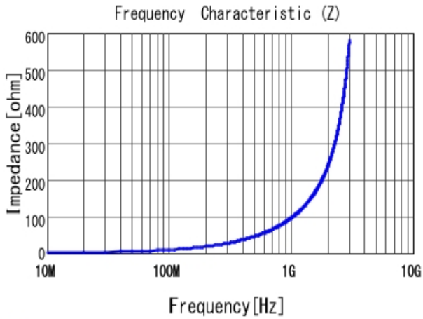
■ LQW2BAS15NJ00 |Z|
