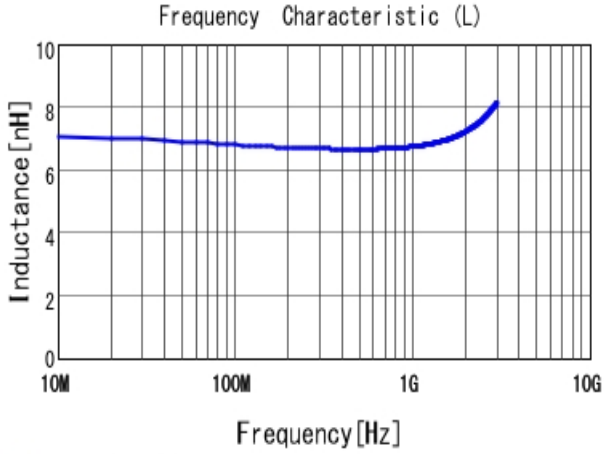
■ LQW2BAS6N8J00 L
