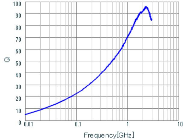
LQW2BAS7N5J00 Q.
