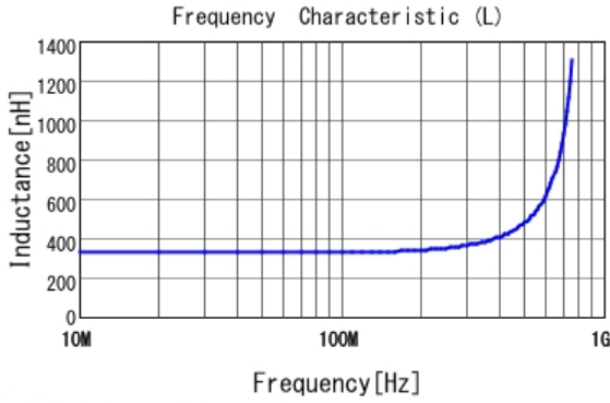
■ LQW2BASR33G00 L
