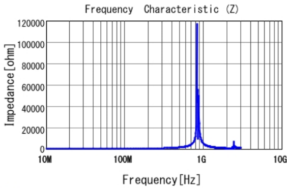
■ LQW2BASR33G00 |Z|
