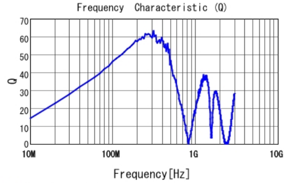
■ LQW2BASR33G00 Q
