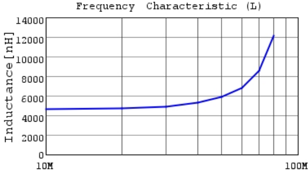
LQW2UAS4R7J0C L
