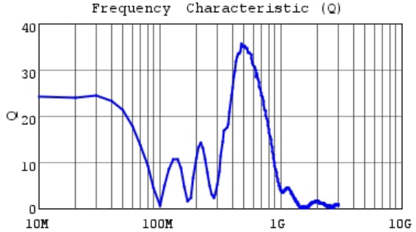
LQW2UAS4R7J0C Q
