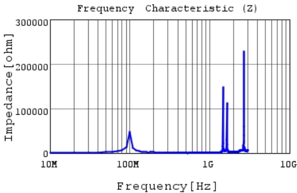
LQW2UAS4R7J0C |Z|
