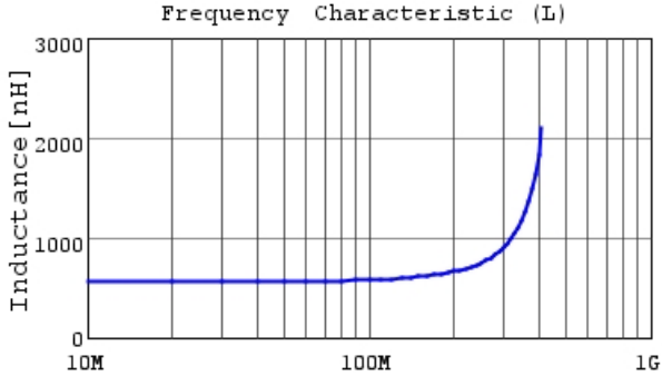
LQW2UASR56G0C L
