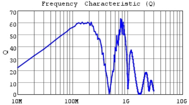
LQW2UASR56G0C Q
