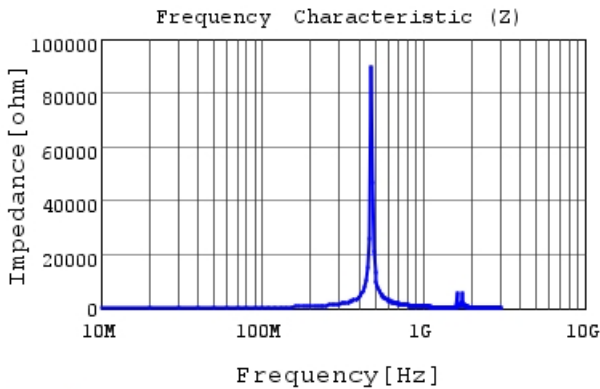
LQW2UASR56G0C |Z|
