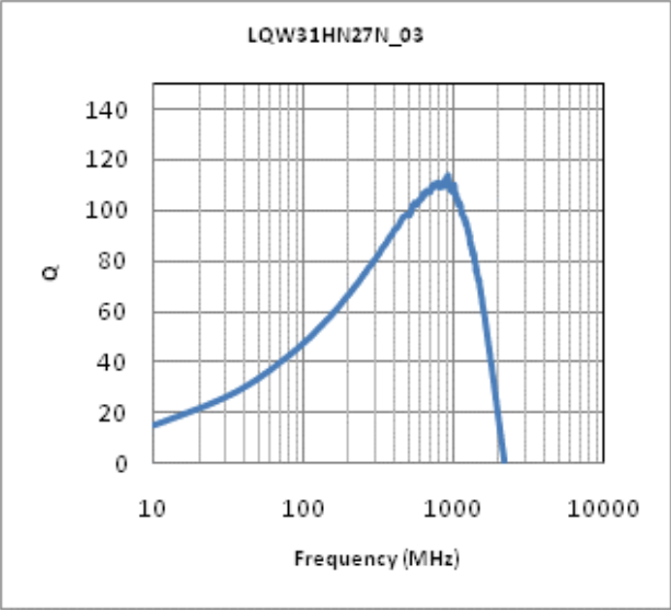
Q-Frequency Characteristics
