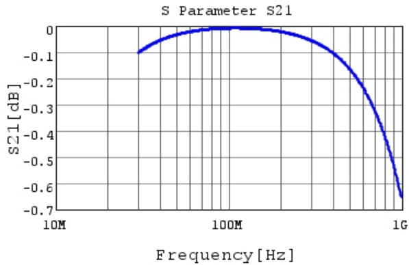
RHE5G1H331J0K1H03B S21 DCOV, 25degC
