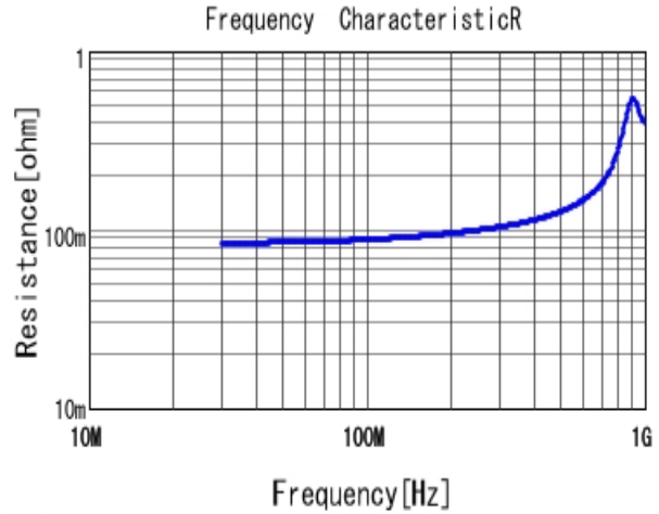
■ RHE5G1H391J0K1H03B R DCOV, 25degC
