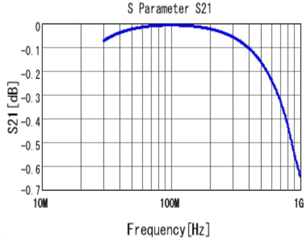
■ RHE5G1H391J0K1H03B S21 DCOV, 25degC
