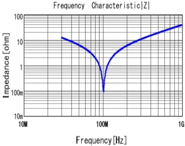
■ RHE5G1H391J0K1H03B |Z| DCOV, 25degC
