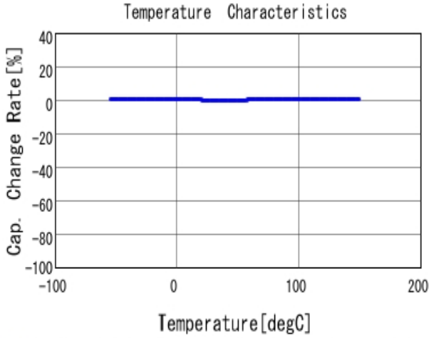
■ RHE5G1H391J0K1H03B C-Temp. capchange, DCOV, AC1Vrms
