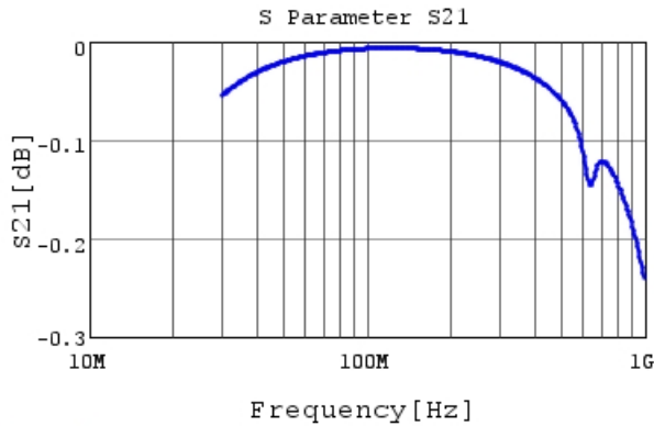
RHE5G2A471J0A2H03B S21 DC0V, 25degC
