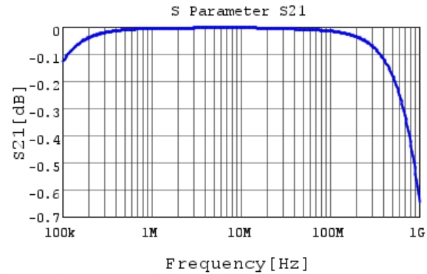
RHEL81E104K0K1H03B S21 DCOV, 25degC
