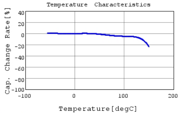
RHEL81E104K0K1H03B C-Temp. capchange, DCOV,
