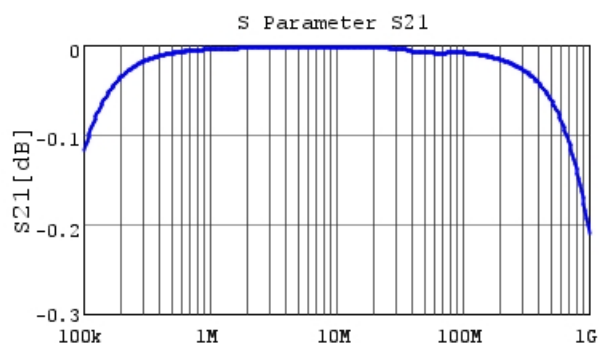
Frequency [Hz] RHEL82A104K1DBH03A S21 DCOV, 25degC
