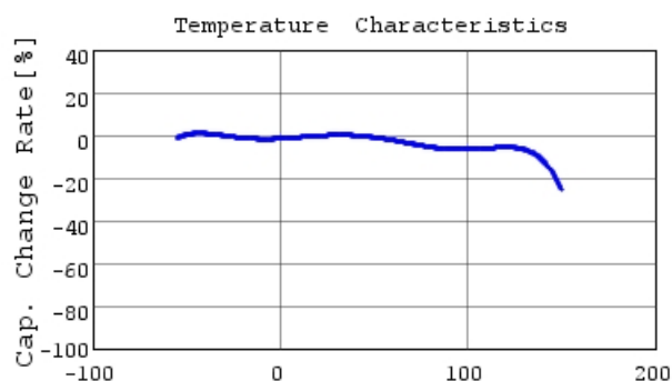
Temperature [degC] RHEL82A104K1DBH03A C-Temp. capchange, DCOV,
