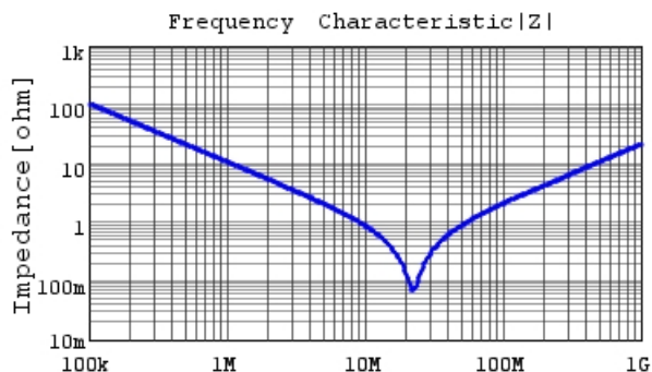
RHEL82A153K0A2H03B |Z| DCOV, 25degC
