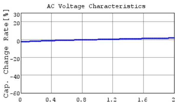
RHEL82A153K0A2H03B C-AC Voltage capchange, 1
