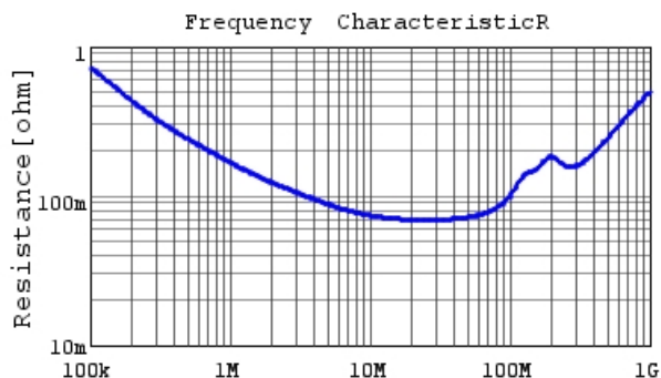
RHEL82A153K0A2H03B R DCOV, 25degC
