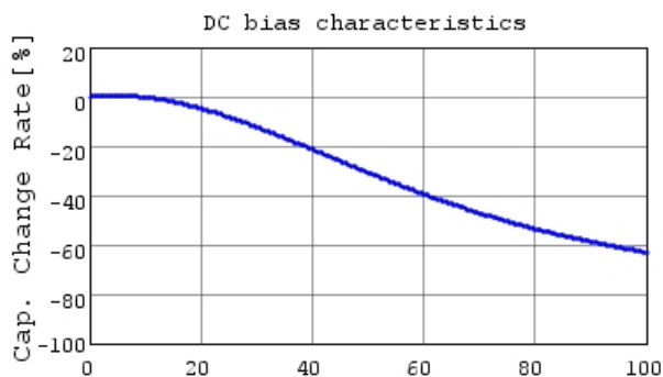
RHEL82A153K0A2H03B C-DC bias capchange, 25.0
