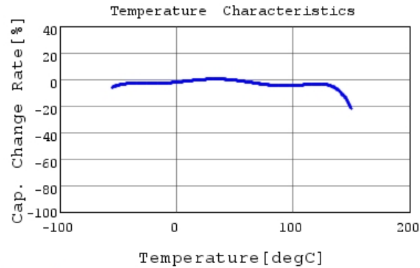
RHEL82A221K0A2H03B C-Temp. capchange, DCOV,
