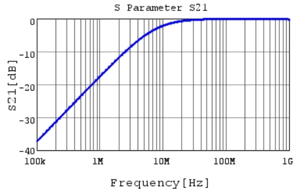
RHEL82A221K0A2H03B S21 DCOV, 25degC
