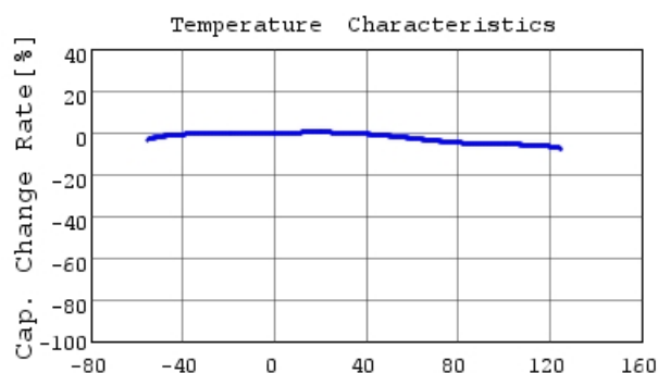
■ GCE188R72A562KA01 C-Temp. capchange, DC0.0V,
