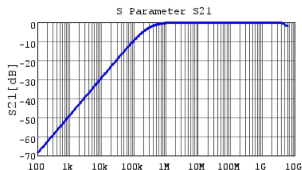
■ GCE188R72A562KA01 S21 DC0V, 25degC
