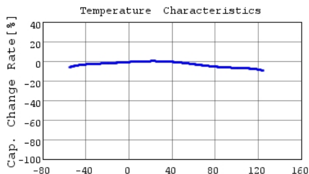
Temperature [degC] GCE21BR71H153KA01 C-Temp. capchange, DC0.0V,
