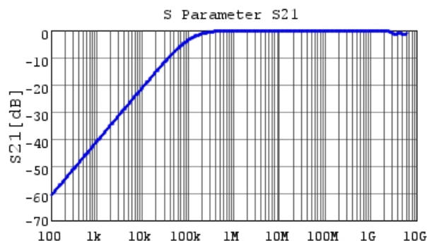
Frequency [Hz] GCE21BR71H153KA01 S21 DC0V, 25degC
