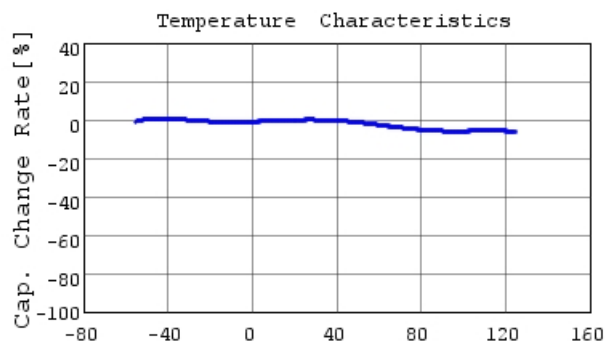
Temperature [degC] GCJ188R72A102KA01 C-Temp. capchange, DC0.0V,
