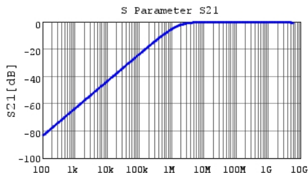
Frequency [Hz] GCJ188R72A102KA01 S21 DC0V, 25degC
