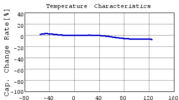
■ GCJ188R72A103KA01 C-Temp. capchange, DC0.0V,
