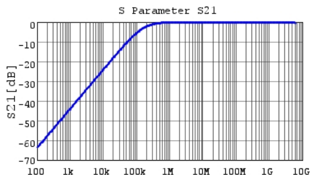
■ GCJ188R72A103KA01 S21 DC0V, 25degC
