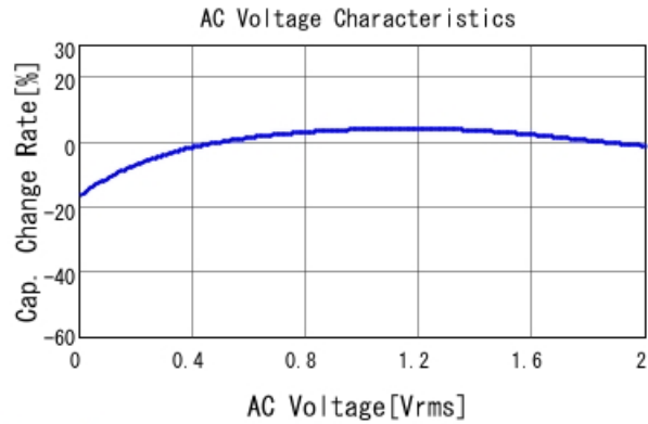
GCM033D70E105ME36 C-AC Voltage capchange, DCOV, 25
