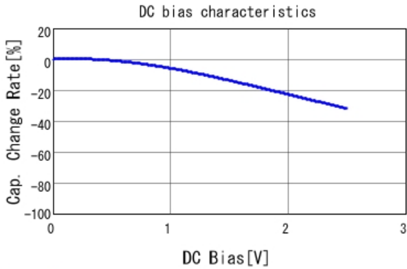
GCM033D70E105ME36 C-DC bias capchange, 25.0degC, A
