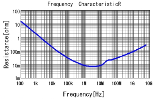
GCM033D70E105ME36 R DCOV, 25degC
