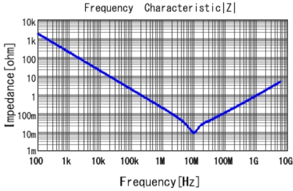
GCM033D70E105ME36 |Z| DCOV, 25degC
