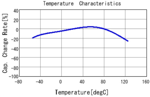
GCM033D70E105ME36 C-Temp. capchange, DC0.0V, AC0.C
