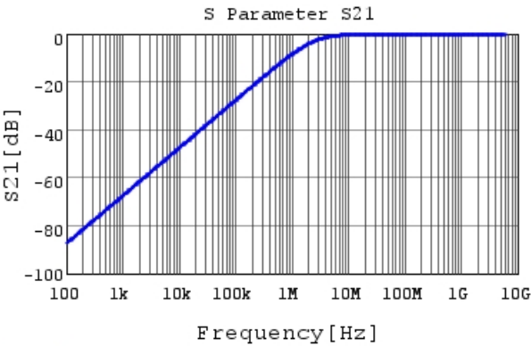
GCM033R71E681KA03 S21 DC0V,25degC
