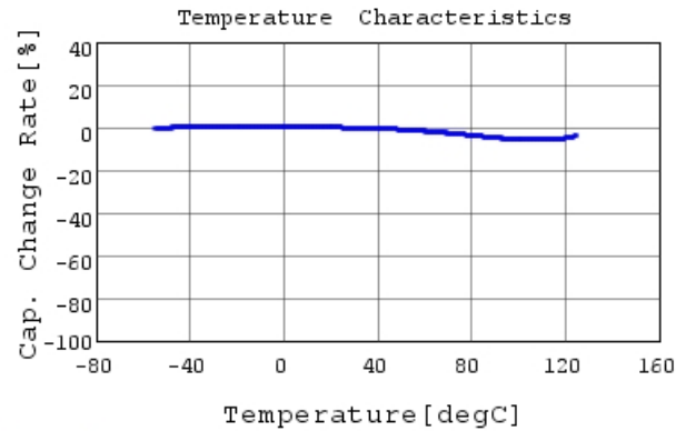
GCM033R71E681KA03 C-Temp. capchange, DC0.0V,
