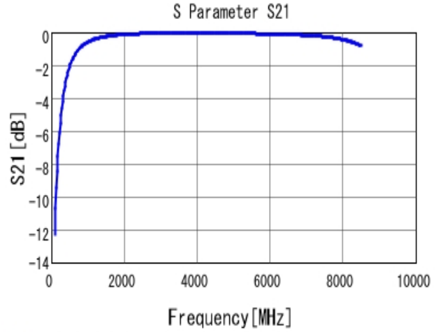
■ GCM1555C1H4R0CA16 S21 DCOV, 25degC
