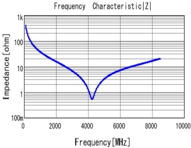
GCM1555C1H4R0CA16 |Z| DCOV, 25degC
