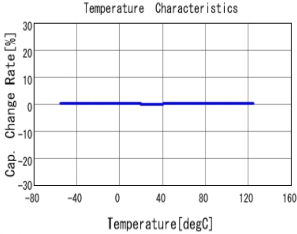
■ GCM1555C1H4R0CA16 C-Temp. capchange, DCOV, AC1Vrms
