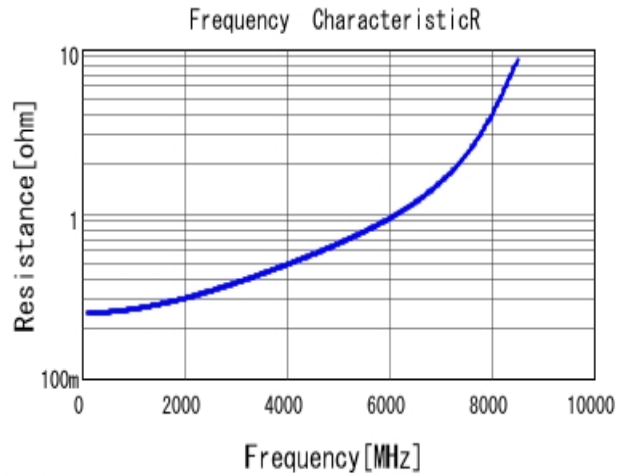
GCM1555C1H4R0CA16 R DCOV, 25degC
