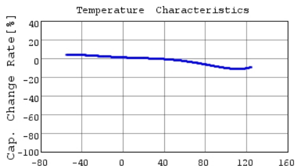
■ GCM155R72A332KA37 C-Temp. capchange, DC0.0V,
