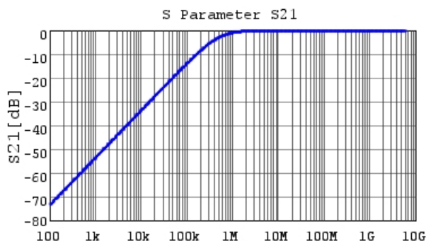
■ GCM155R72A332KA37 S21 DC0V, 25degC
