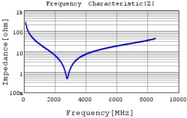
GCM1885C2A6R0DA16 |Z| DCOV,25degC
