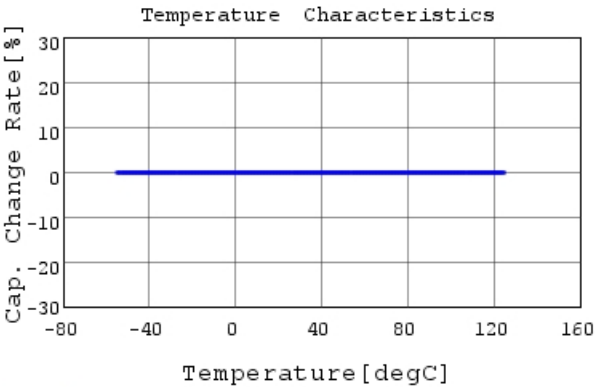
GCM21A5C2E272GX01 C-Temp. capchange, DC0V, 1
