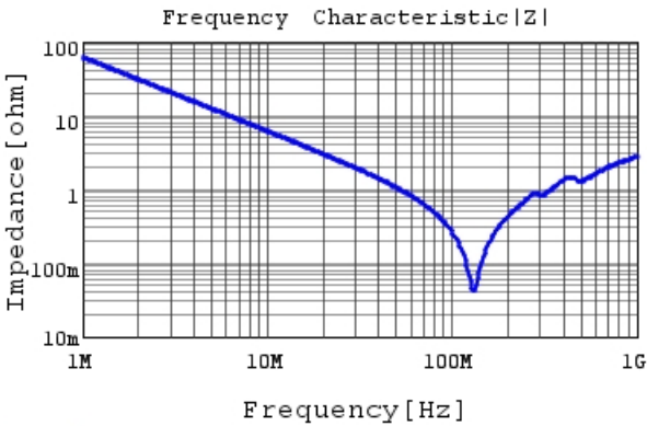
GCM21A5C2E272GX01 |Z| DC0V, 25degC
