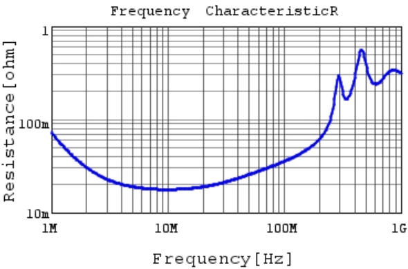
GCM21A5C2E272GX01 R DC0V, 25degC
