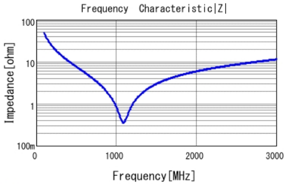
■ GCM21A5C2E330JX01 |Z| DC0V, 25degC
