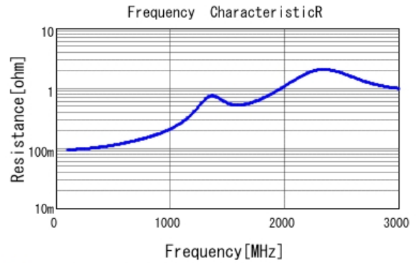
■ GCM21A5C2J181JX01 R DC0V, 25degC
