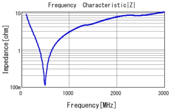
■ GCM21A5C2J181JX01 |Z| DC0V, 25degC
