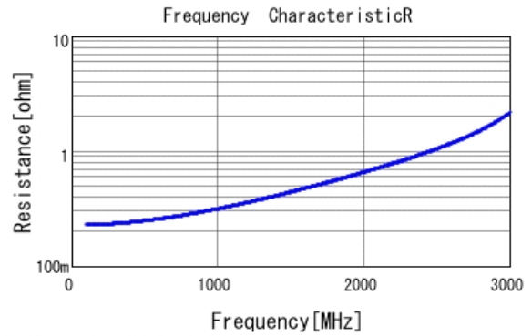
■ GCM31A5C3A220JX01 R DC0V, 25degC
