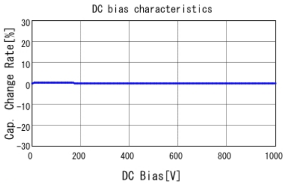
■ GCM31A5C3A220JX01 C-DC bias capchange, 25.0degC, AC1V
