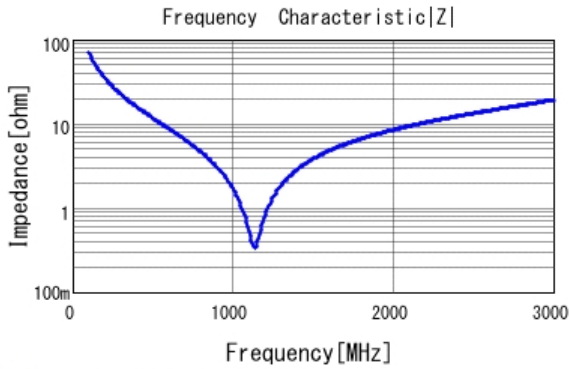
■ GCM31A5C3A220JX01 |Z| DC0V, 25degC
