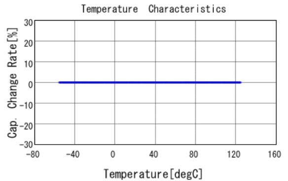
■ GCM31A5C3A220JX01 C-Temp. capchange, DC0V, AC1Vrms
