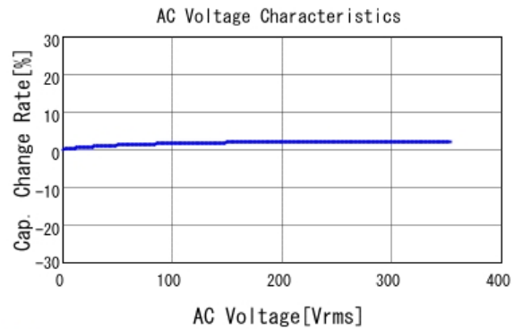
■ GCM31A7U3A120JX01 C-AC Voltage capchange, DC0V, 25.0d
