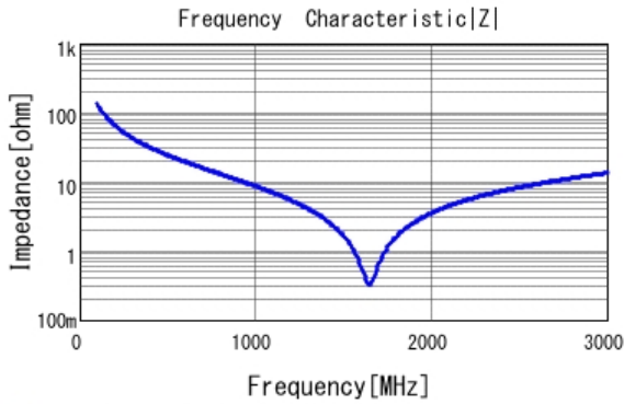
■ GCM31A7U3A120JX01 |Z| DC0V, 25degC
