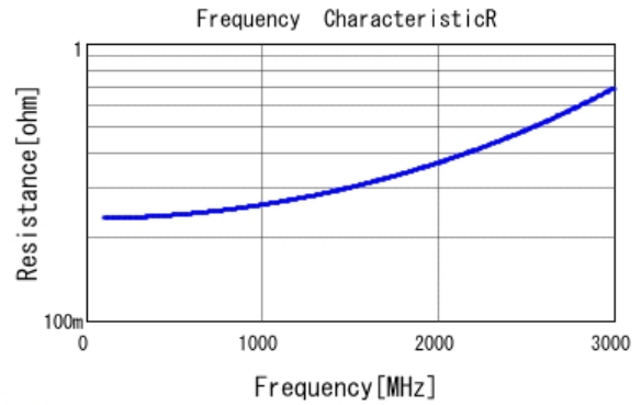
■ GCM31A7U3A120JX01 R DC0V, 25degC
