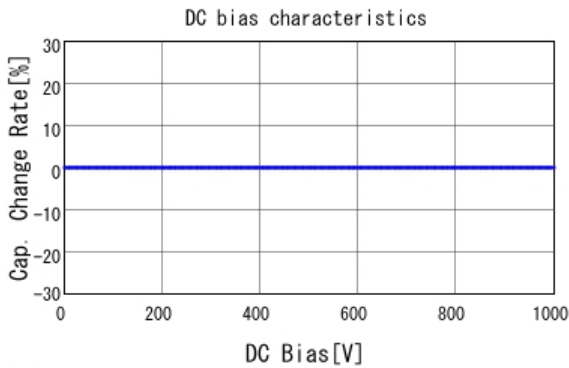
■ GCM31A7U3A120JX01 C-DC bias capchange, 25.0degC, AC1V
