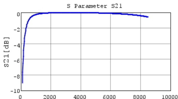
■ GJM1555C1H6R0BB01 S21 DCOV, 25degC
