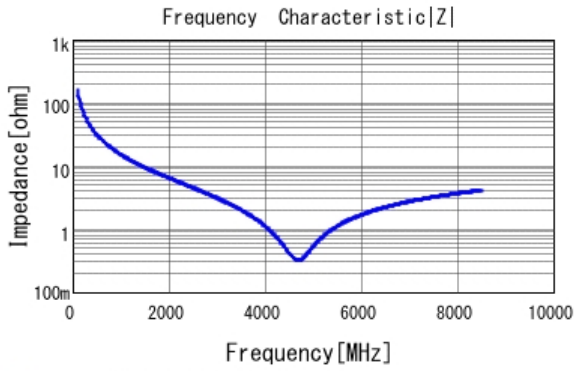
■ GRM0115C1E100GE01 |Z| DCOV, 25degC
