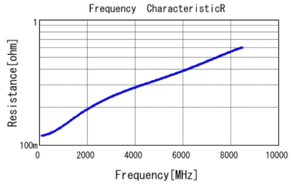
■ GRM0115C1E100GE01 R DCOV, 25degC
