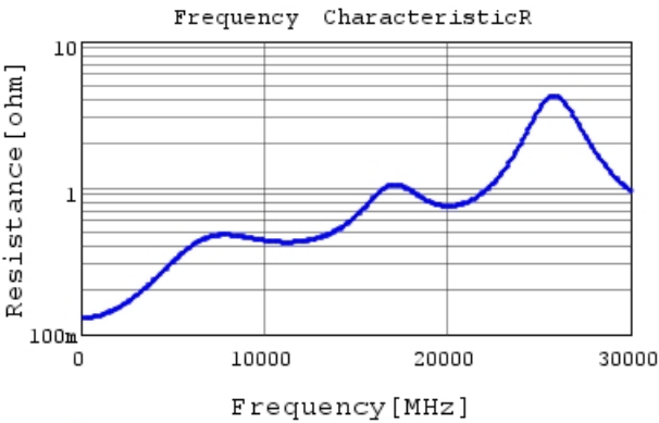
GRM0115C1E7R0WE01 R DCOV,25degC
