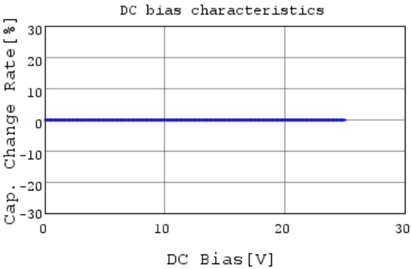
GRM0115C1E7R0WE01 C-DC bias capchange, 25.0C
