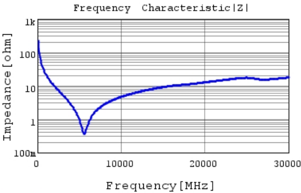
GRM0115C1E7R0WE01 |Z| DCOV,25degC
