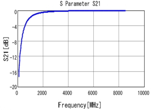
■ GRM0223C1H2R2WA03 S21 DCOV, 20degC
