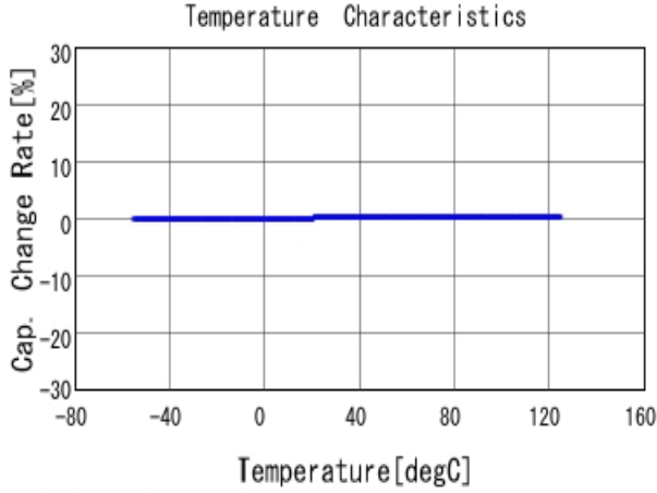
■ GRM0223C1H2R2WA03 C-Temp. capchange, DCOV, AC1Vrms
