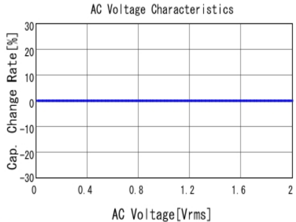
■ GRM0223C1H2R2WA03 C-AC Voltage capchange, DC0V, 20.0d
