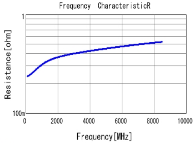
■ GRM0223C1H2R2WA03 R DC0V, 20degC
