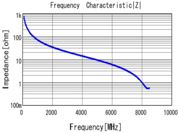
■ GRM0223C1H2R2WA03 |Z| DC0V, 20degC
