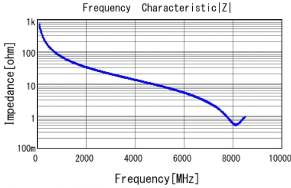
■ GRM0223C1H2R3CA03 |Z| DCOV, 20degC
