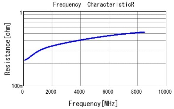
■ GRM0223C1H2R3CA03 R DCOV, 20degC
