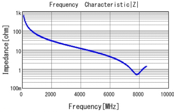
■ GRM0223C1H2R5WA03 |Z| DCOV, 20degC
