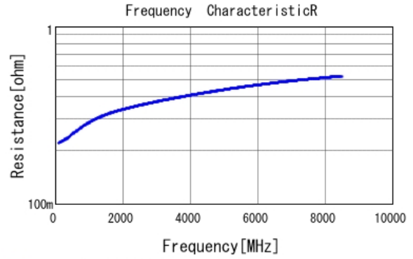
■ GRM0223C1H2R5WA03 R DCOV, 20degC
