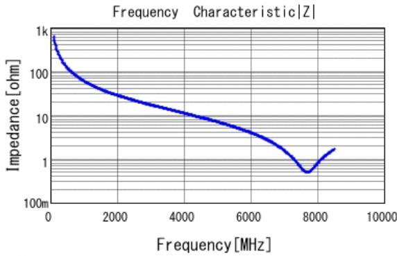
■ GRM0223C1H2R6BA03 |Z| DCOV, 20degC
