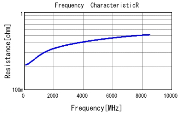
■ GRM0223C1H2R6BA03 R DCOV, 20degC
